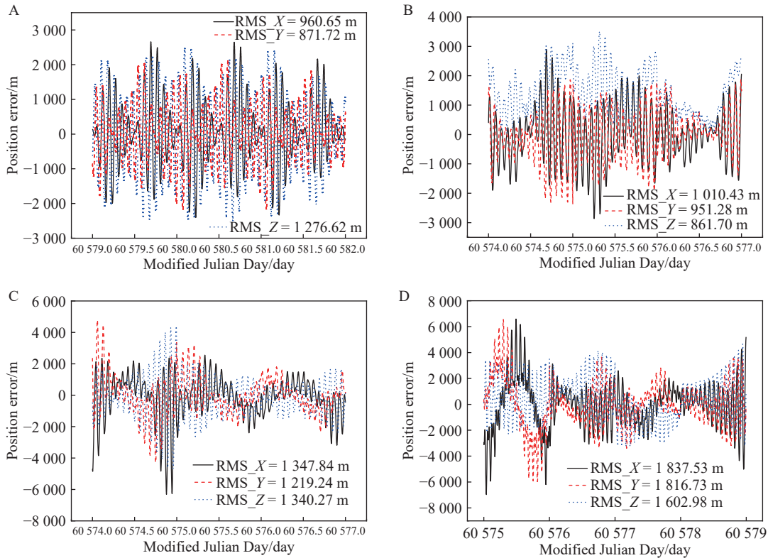
Fig. 6. Position error comparing OD results with TLE data: (A) target for 21233, (B) target for 45535, (C) target for 58377, and (D) target for 60264.
