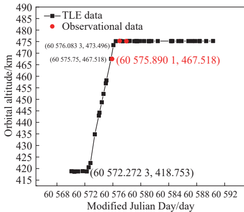
Fig. 8. Orbital altitude of NORAD number 60439 over time as shown by TLE data and observational data.
