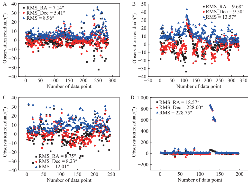
Fig. 5. Observation residual of target after OD: (A) target for 21233, (B) target for 45535, (C) target for 58377, and (D) target for 60264.
