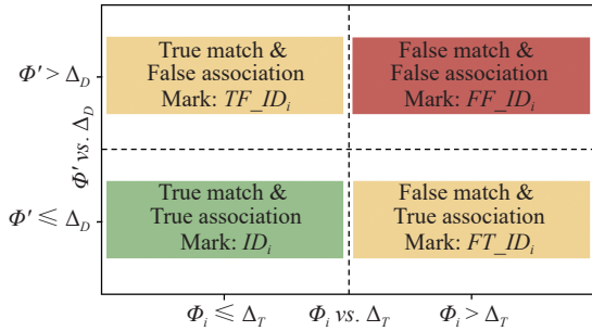
Fig. 1. Diagram of matching and association relationship.
