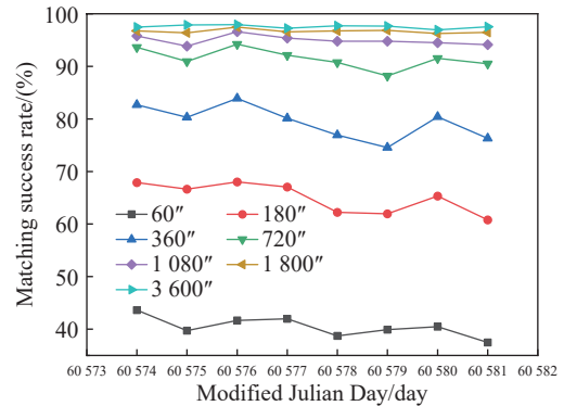
Fig. 4. Matching success rate at different matching error thresholds.
