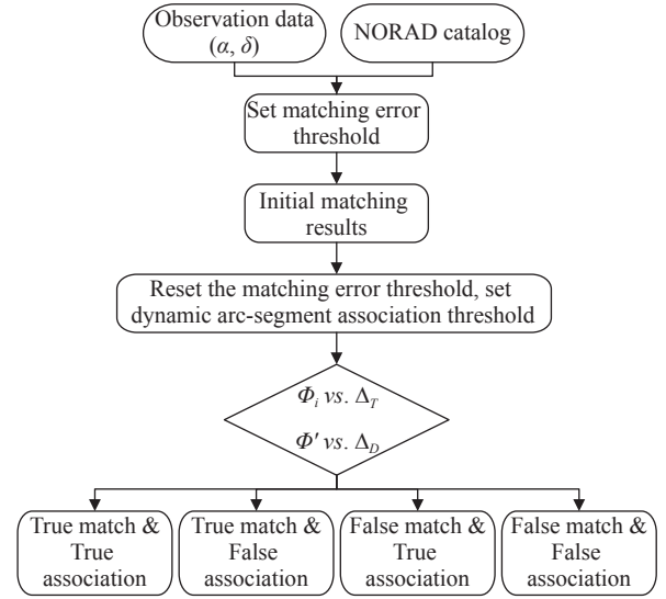
Fig. 2. Flow chart of the process of data matching and association processing.
